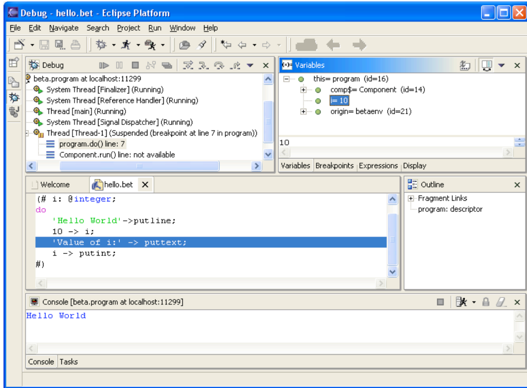
Fig. 2. Debugging BETA in Eclipse
