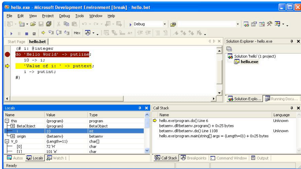
Fig. 3. Debugging BETA in Visual Studio .NET
