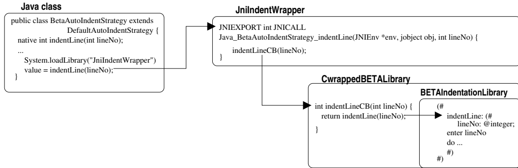
Fig. 1. Java BETA interoperability using JNI
