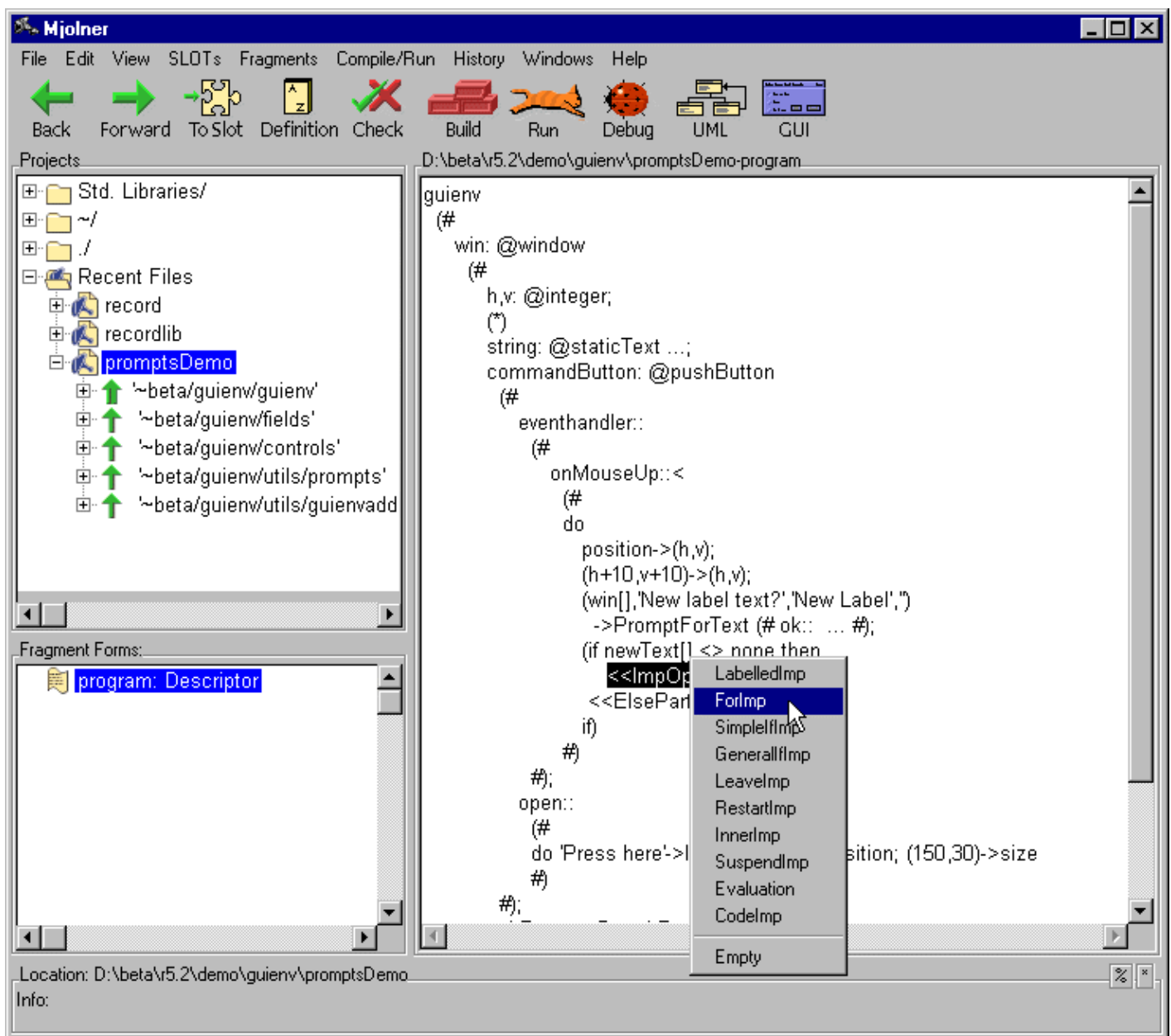
Figure 1: Source browser and editor
