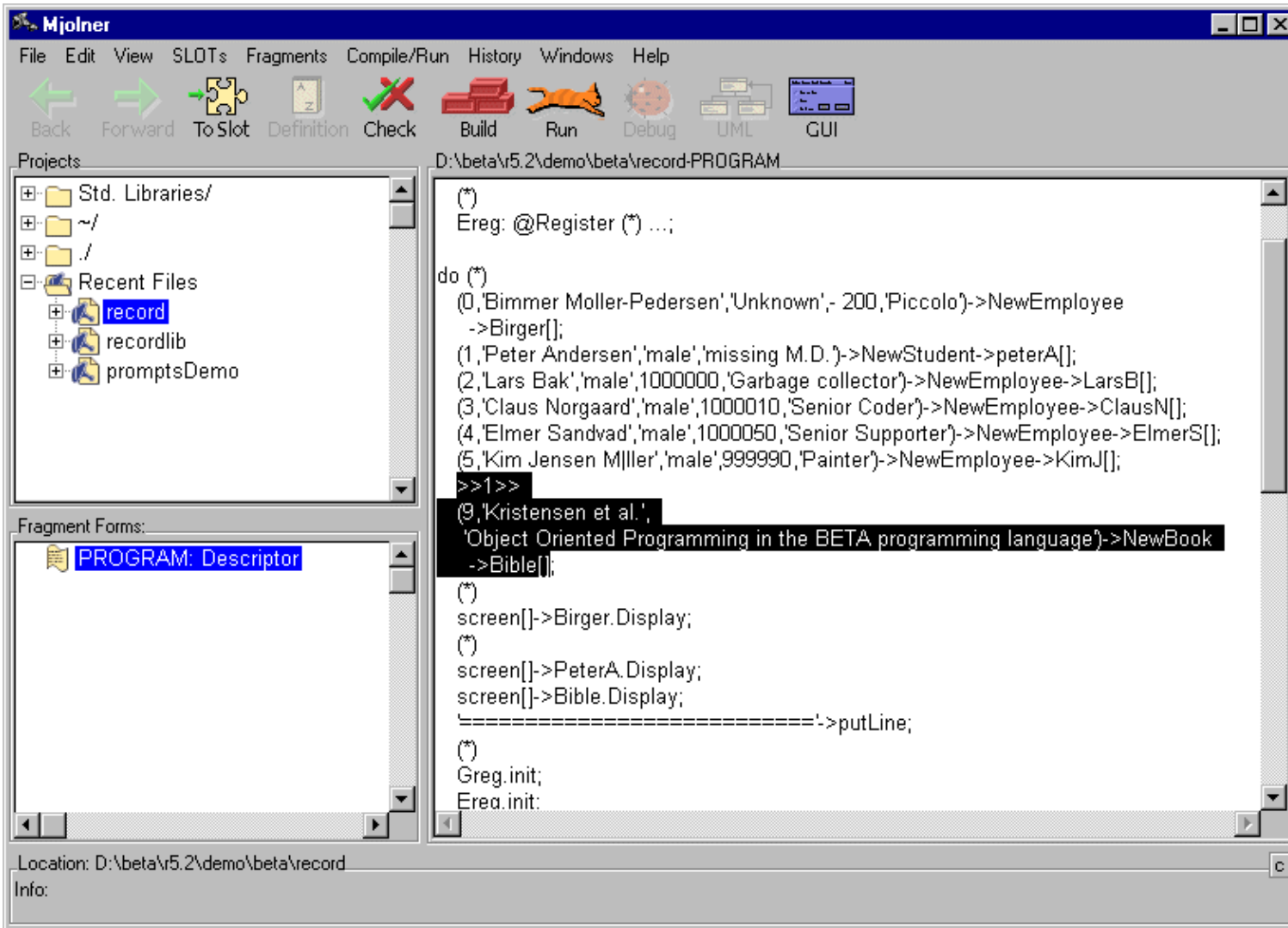
Figure 3: A breakpoint
