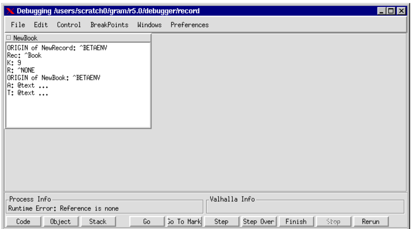
Figure 2: Debugger universe
